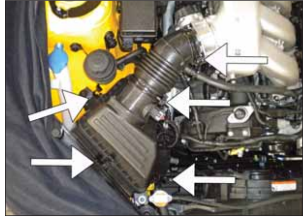
b. Unclip the four airbox clips and loosen the clamp at the throttle body. Unplug the MAF sensor.
