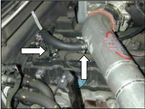
i. Attach the supplied 1/2" hose between the intake pipe and the valve cover inlet as shown. Trim to fit and secure using the supplied hose clamps.
