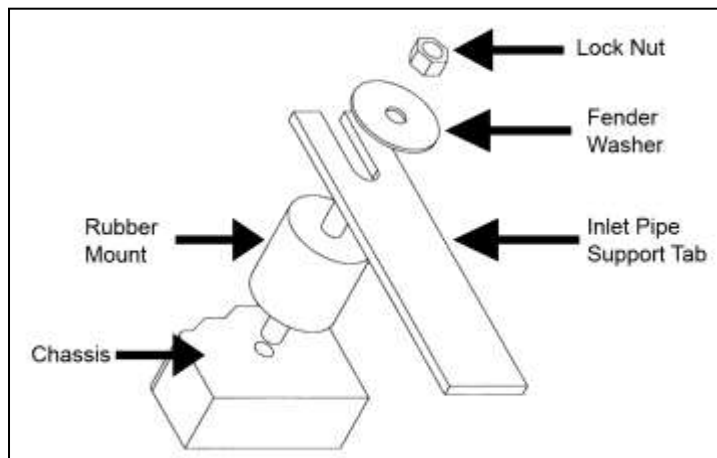
Proper installation of rubber mount assembly.
