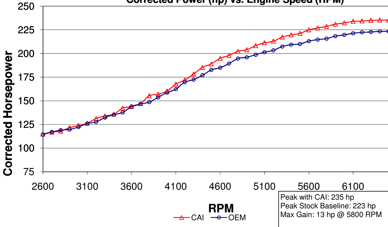
Corrected Power (hp) vs. Engine Speed (RPM)
