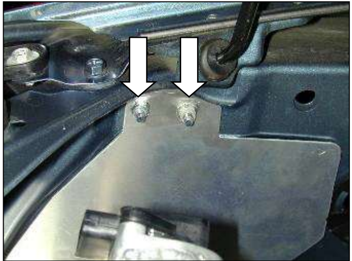
g. Place the heat shield over the intake pipe. Secure the heat shield to the upper two mounting studs left by the air box bracket.
